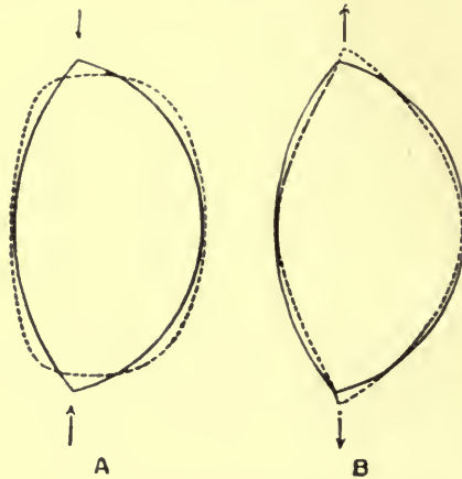
FIG. 105.—Lens of the ox, twice enlarged. The dotted line indicates the form which the crystalline lens assumes : (A) by a lateral pressure (B) by traction exerted on the zonula. The arrows indicate the direction of the forces (Tscherning).
